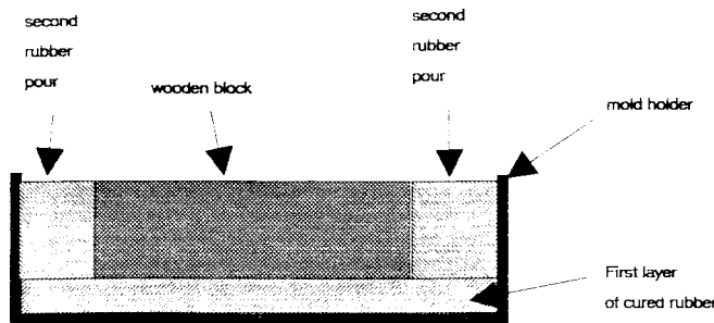
FIG. X1.1 Cross Section View of Materials Used to Prepare a Silicone Rubber Mold for Coal Blocks
