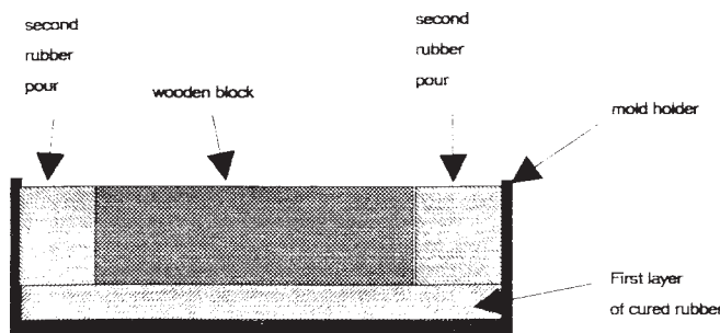
FIG. X1.1 Cross Section View of Materials Used to Prepare a Silicone Rubber Mold for Coal Blocks
