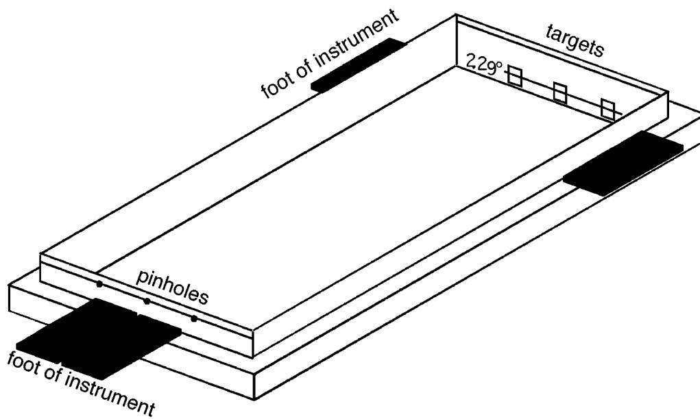
FIG. 4 Frame with Pinholes and Targets for Alternative Testing of the Co-viewing Angle and the Aperture for Only the Collimated Instruments
