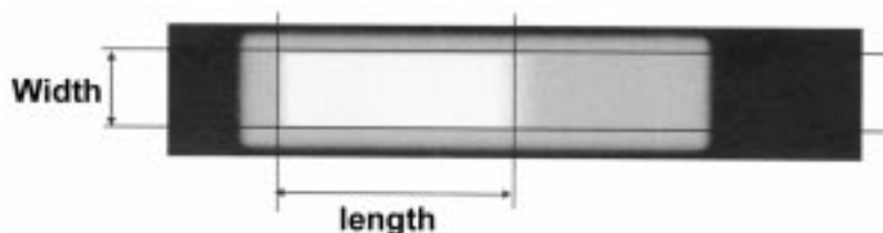
FIG. 5 With Light through the Aperture Stop at the Detector, the Measurement and Illuminated Areas are Projected onto a Plate against the Feet of the Instrument. The Smaller Area is Measured from “Middle of Blur” to “Middle of Blur”
