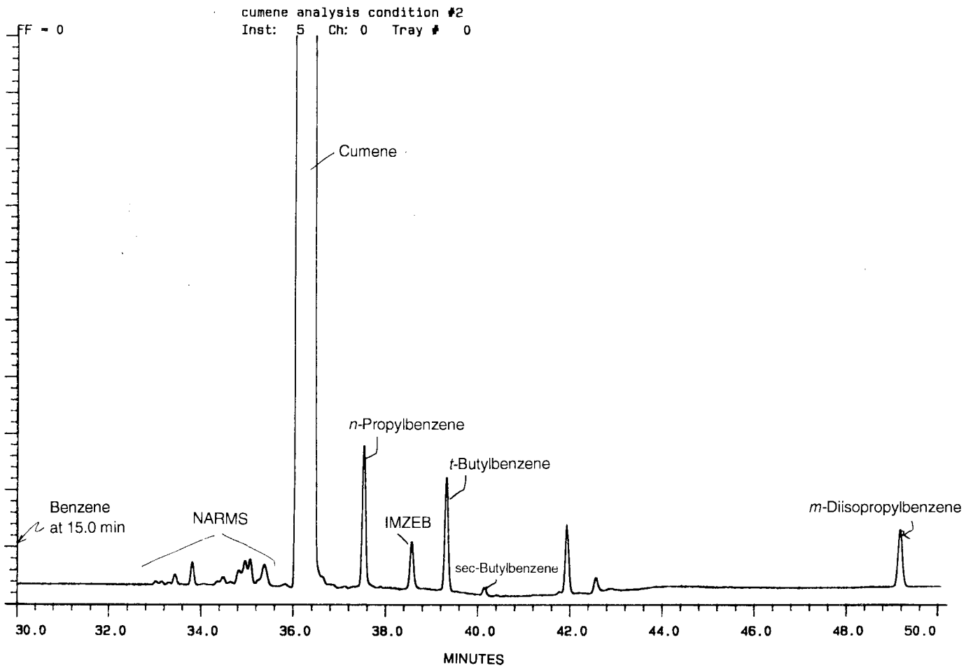
FIG. 2 Typical Chromatogram using Conditions for Column B
