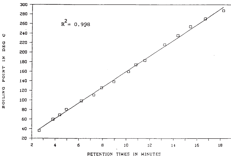
FIG. 3 Calibration Curve
