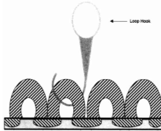
Arrangement of Loop Hook for Loop Pile
