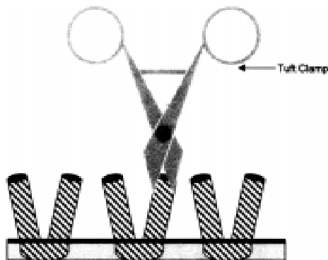
Arrangement of Tuft Clamp for Cut Pile
