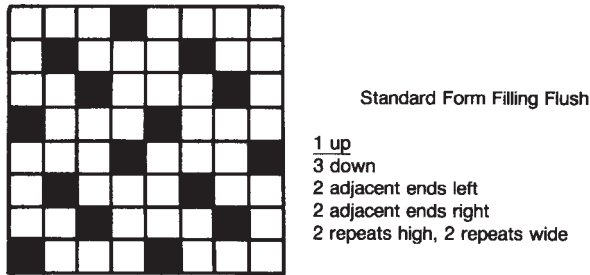
FIG. A1.1 Crowfoot
