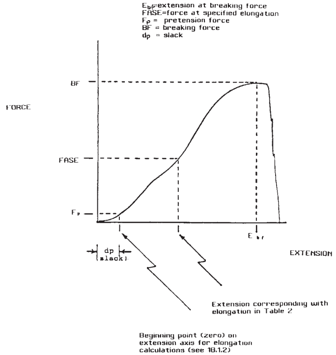
FIG. 1 Force-Extension Curve
