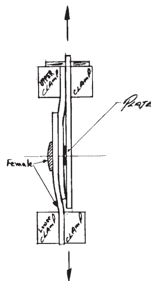
FIG. 4 Specimen Clamping for Lateral Holding Strength
