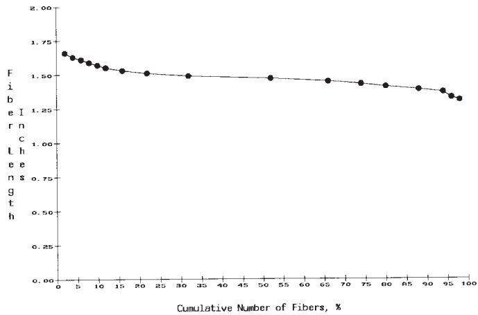
FIG. 2 Example Tally of Measured Fibers, in.
