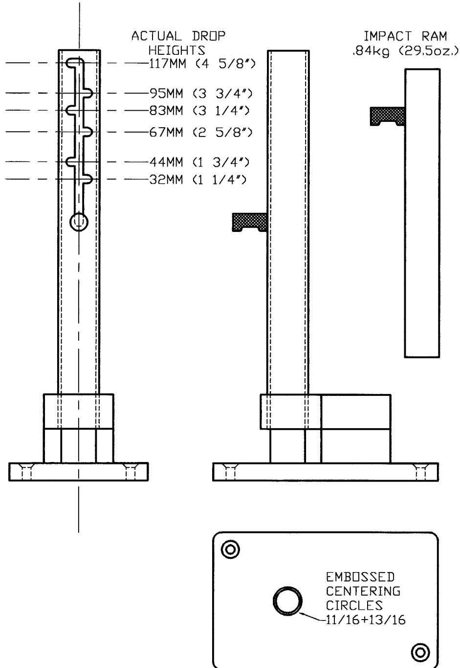
FIG. 1 Impact-Resistance Tester
