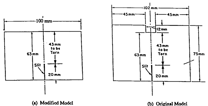
NOTE 1—All tolerances ± 0.5 %. FIG. 1 Example of Die For Cutting Notched Specimens
