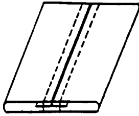
FIG. 266 Stitching Type EFs-2
