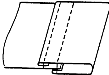
FIG. 168 Seam Type LSbe-2
