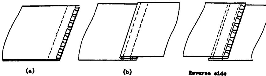
Seam type LSbm-4
