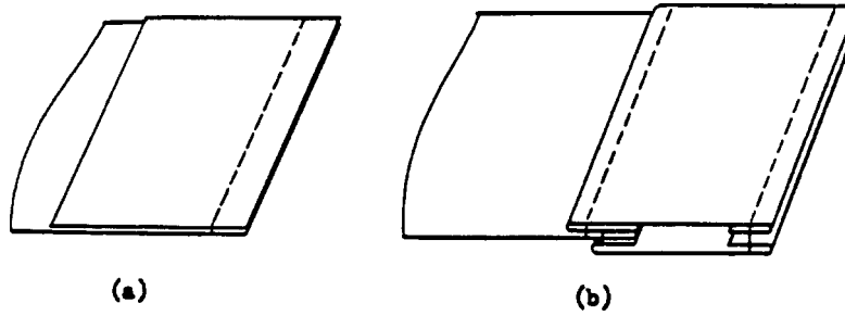
FIG. 200 Seam Type LScm-3
