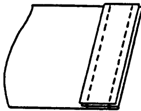
Seam type SSe-2
