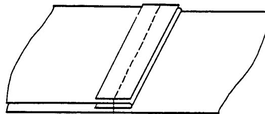
Seam type LSbe-1
