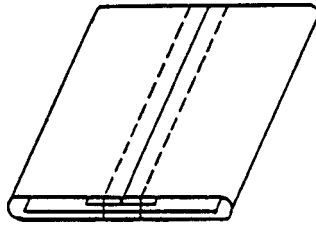
FIG. 276 Stitching Type EFac-2
