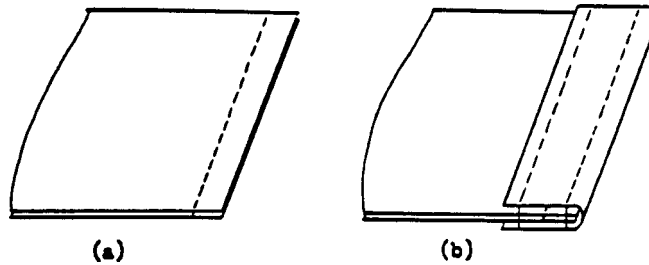
FIG. 224 Seam Type BSg-2
