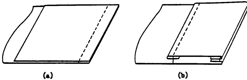
FIG. 206 Seam Type LScs-2
