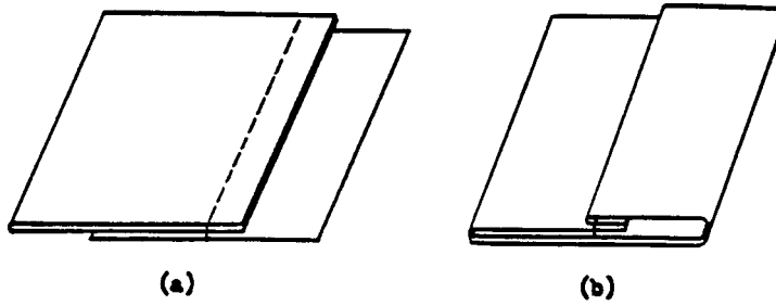
Seam type SSas-1
