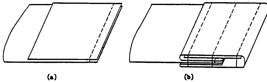
FIG. 229 Seam Type BSm-3
