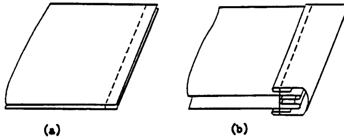
FIG. 232 Seam Type BSp-2
