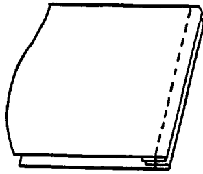
Seam type 3Sc-1
