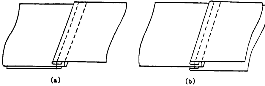
Seam type LSf-2
