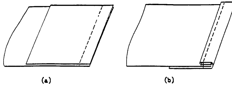
FIG. 231 Seam Type BSo-2
