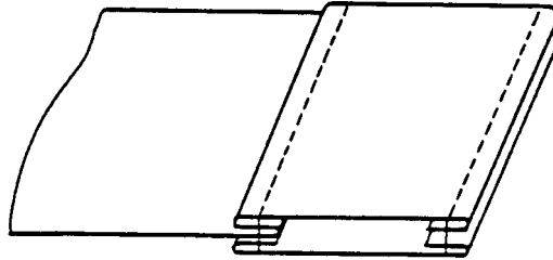
Seam type L3al-2
