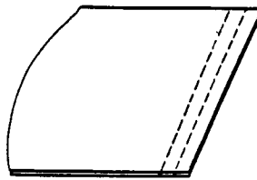
Seam type SSa-2 (Produced with stitch types 301 or 401)
