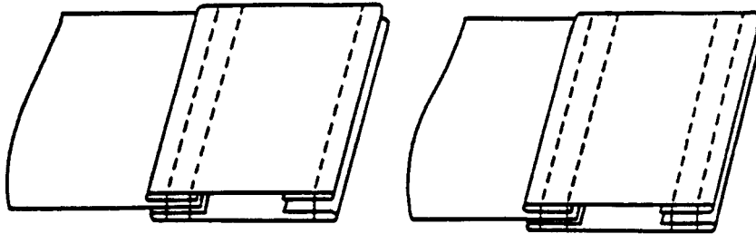
Seam type LSbc-3
