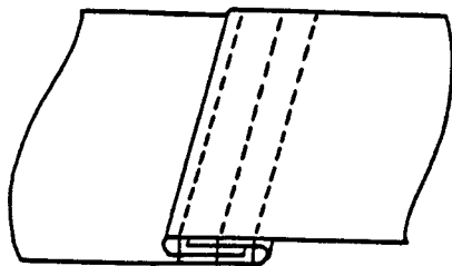
Seam type LSc-3
