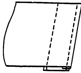
Seam type SSt-2
