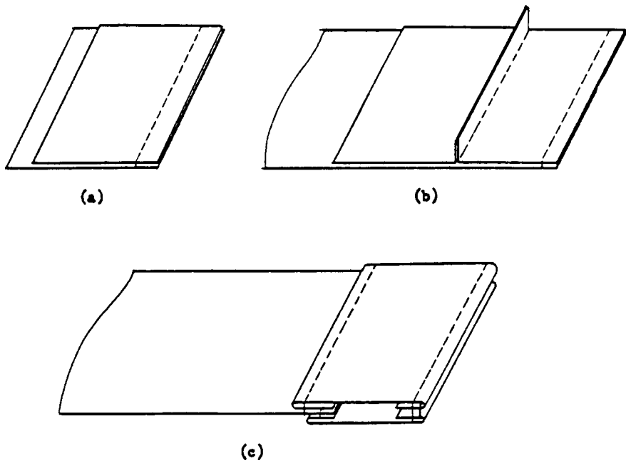
FIG. 202 Seam Type LSco-4
