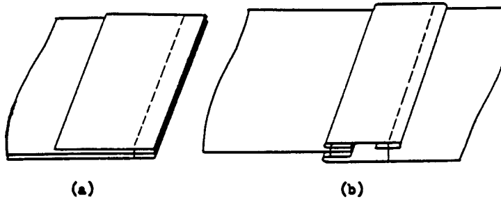
Seam type LSbn-2
