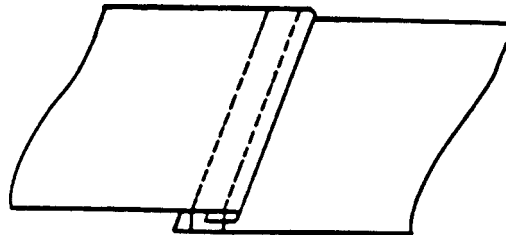
Seam type LSba-2
