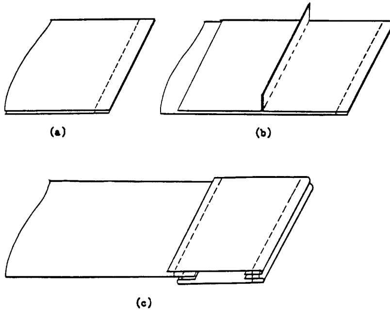
FIG. 204 Seam Type LScq-4
