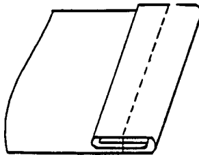
FIG. 269 Stitching Type EFv
