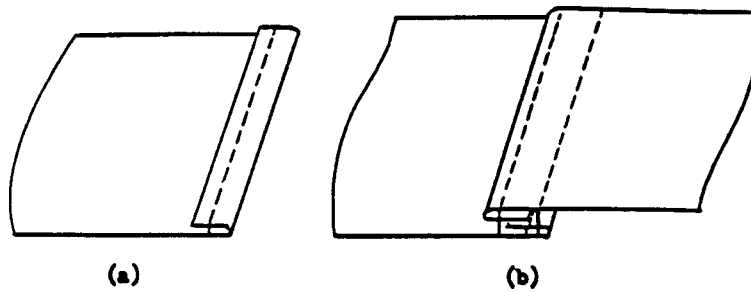
FIG. 215 Seam Type LSdb-2
