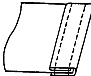
Seam type BSb-2
