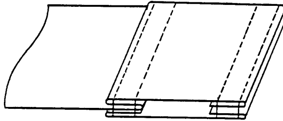
Seam type L3al-4
