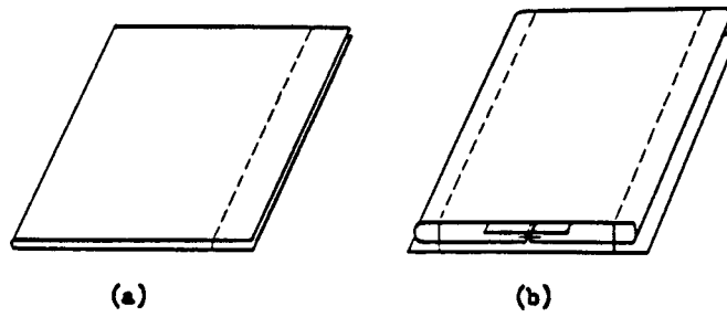
FIG. 209 Seam Type LScv-3
