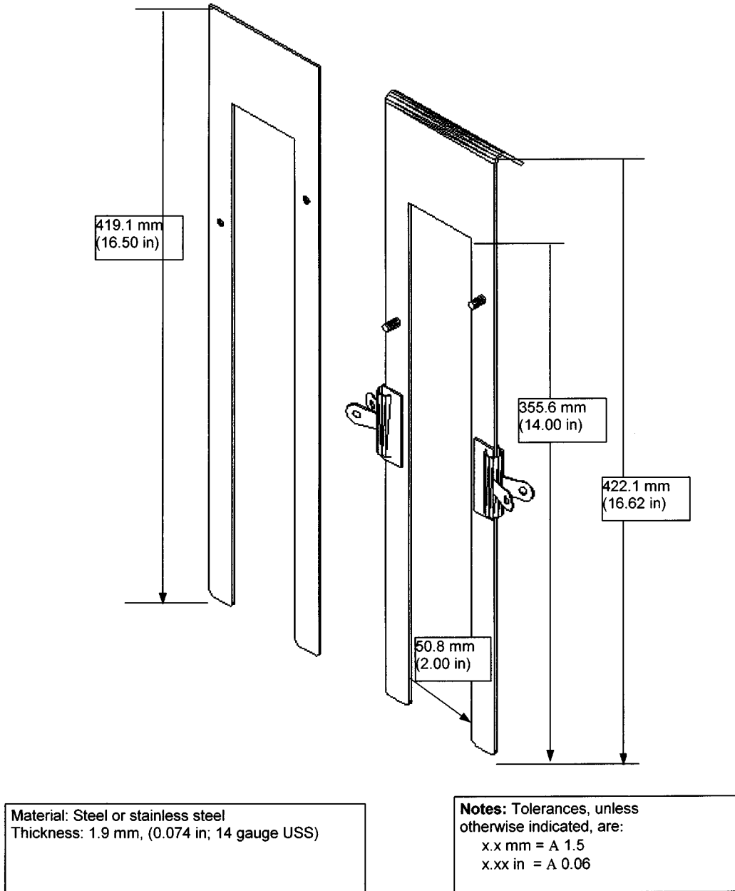
FIG. 5 Flame Height Indicator
