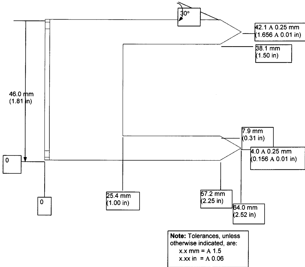
FIG. 6 Sample Holder, Plate (Left) and Frame with Clips
