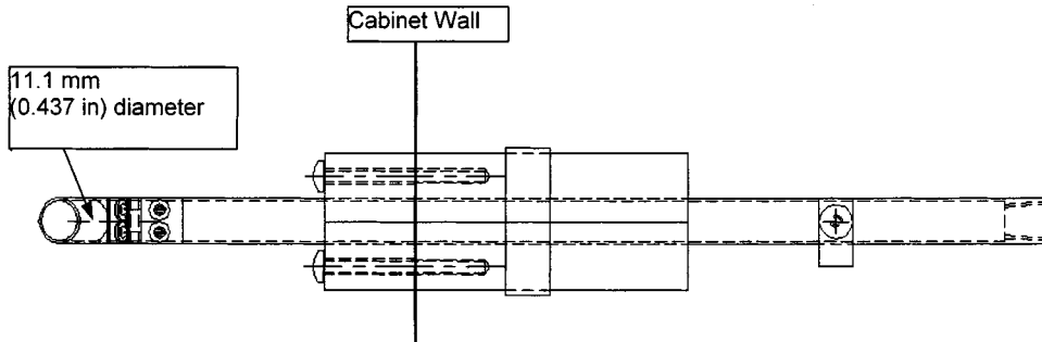
FIG. 8 Burner Arm Assembly (Top View)
