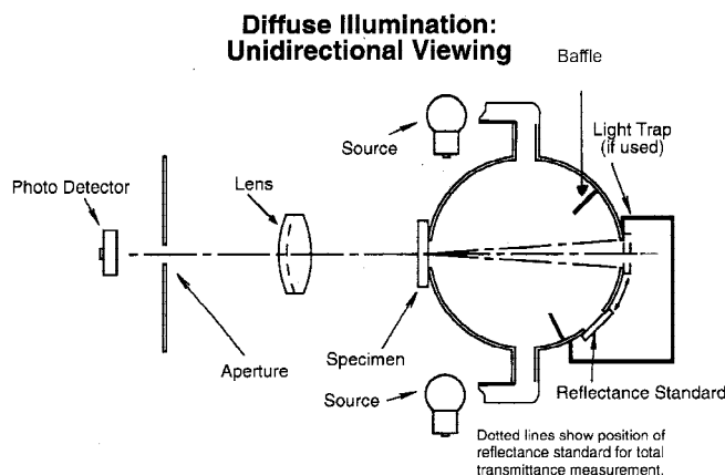
FIG. 2 Spectrophotometer With Diffuse Illumination
