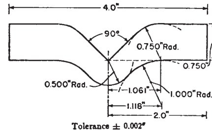
Tolerance \pm 0.002'' Tolerance \pm 0.002'' Tolerance \pm 0.5^\circ Table of Metric Equivalents
