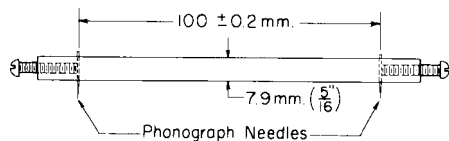
FIG. 1 Scriber
