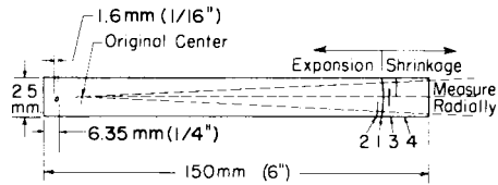
FIG. 1 Scriber
