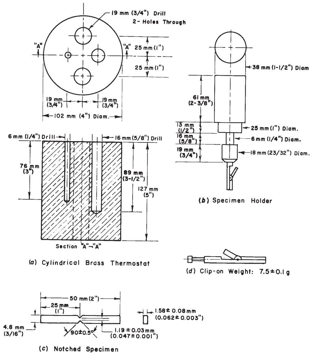
FIG. A1.1 Zero Strength Time Apparatus and Accessories
