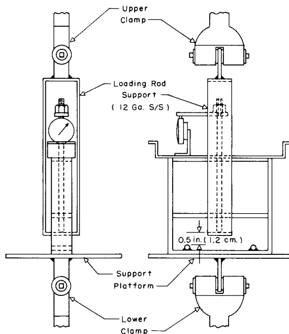
FIG. X2.1 Calibration Apparatus Using a Tensile Machine FIG. X2.1 Calibration Apparatus Using a Tensile Machine
