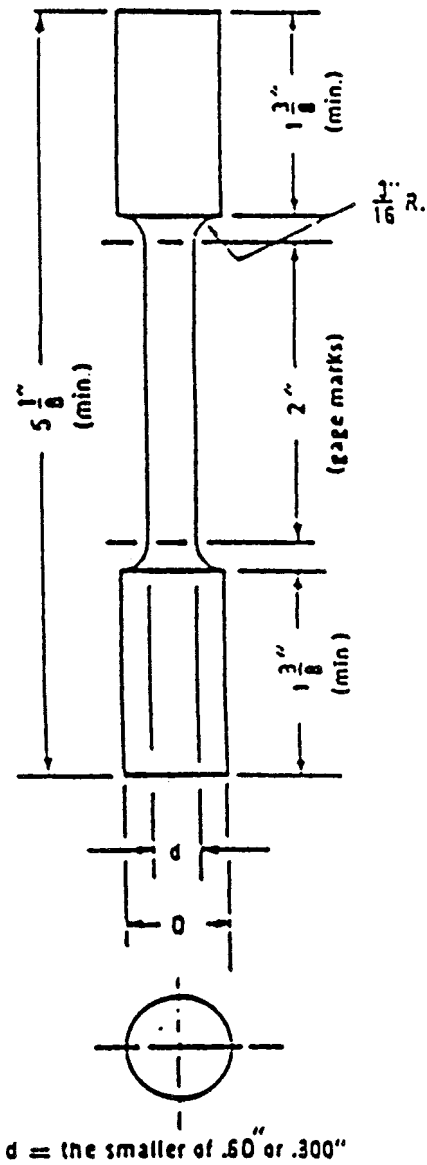
FIG. 1 Turned Dumbbell Specimen for Tensile Testing
