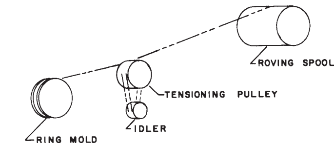
FIG. 4 Schematic Diagram of Preimpregnated Roving Winding System
