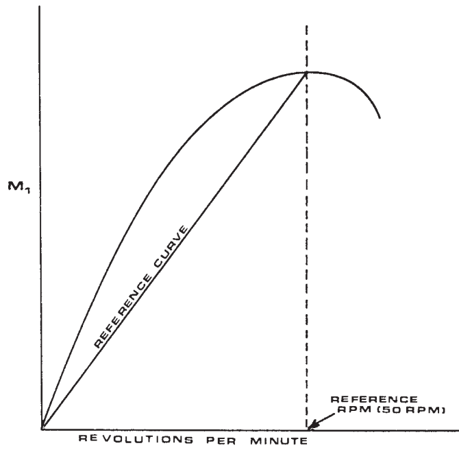
FIG. X1.2 Reference Curve
