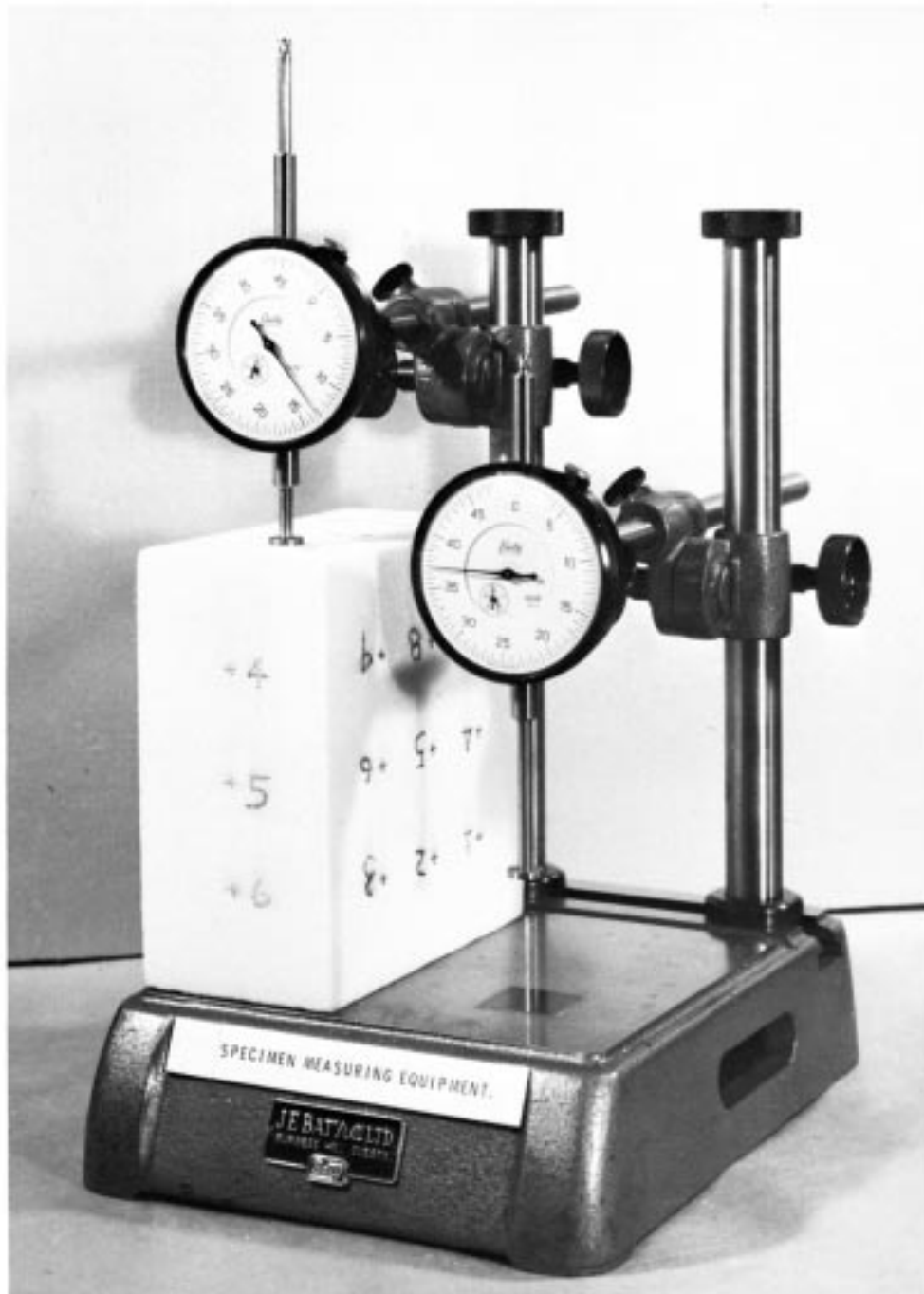
FIG. 2 Dual-Dial Micrometer Measuring Device
