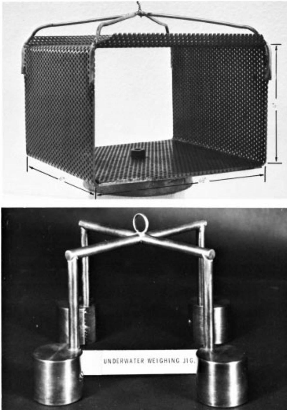
FIG. 1 Underwater Weighing Jigs
