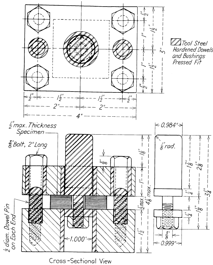
Cross-Sectional View
