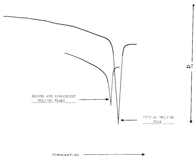
FIG. 5 Melting Characteristics by Thermal Analysis
