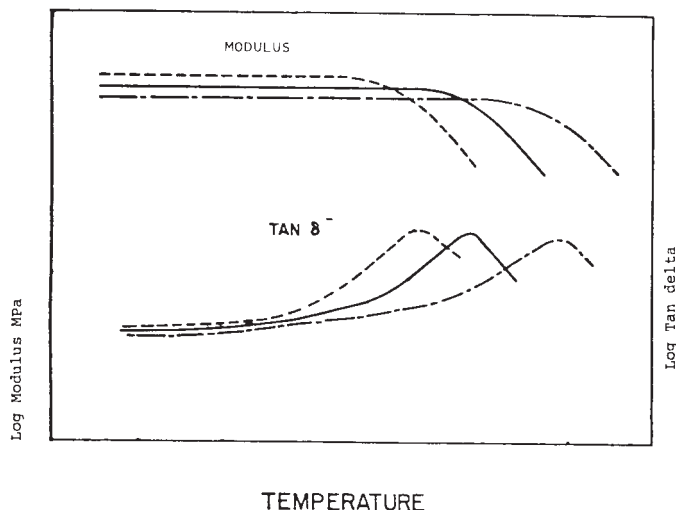
FIG. 1 Dynamic Mechanical Properties in Tension (at Different Frequencies)
