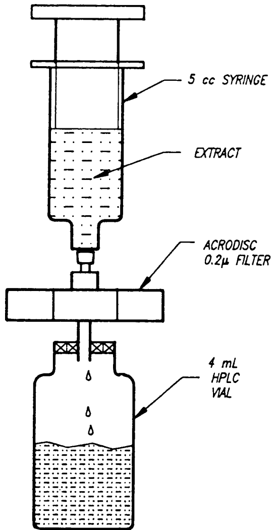
FIG. X1.2 Final Preparation of Sample Extract
