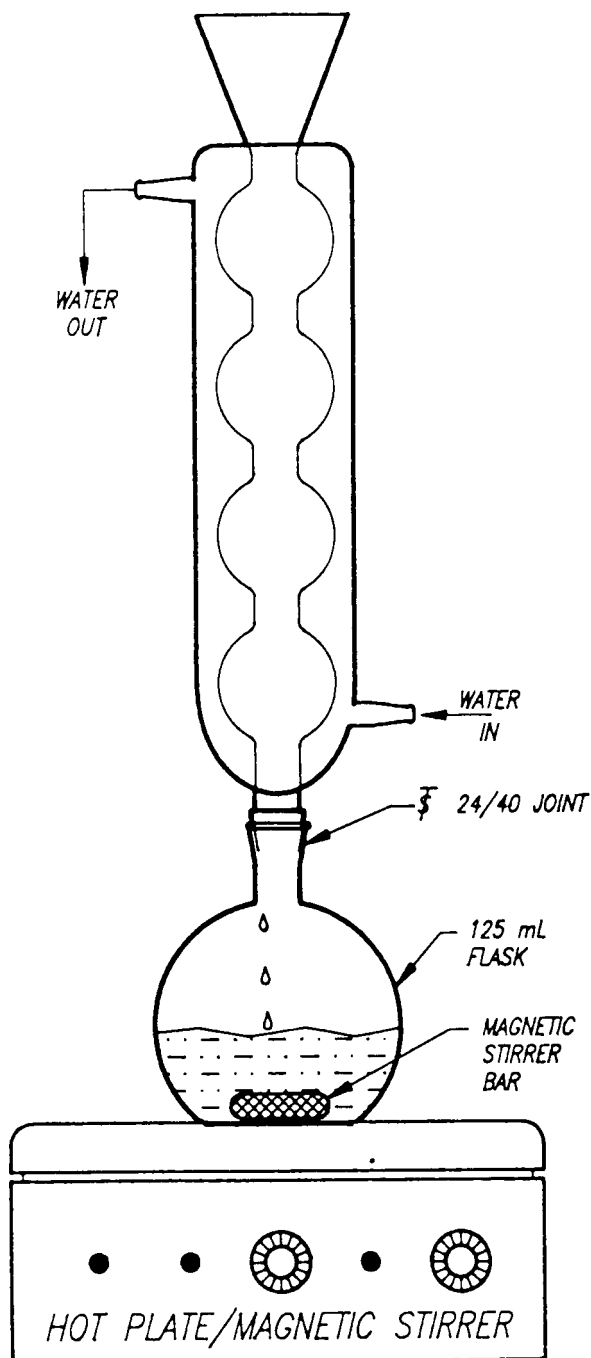
FIG. X1.1 Sample Extraction
