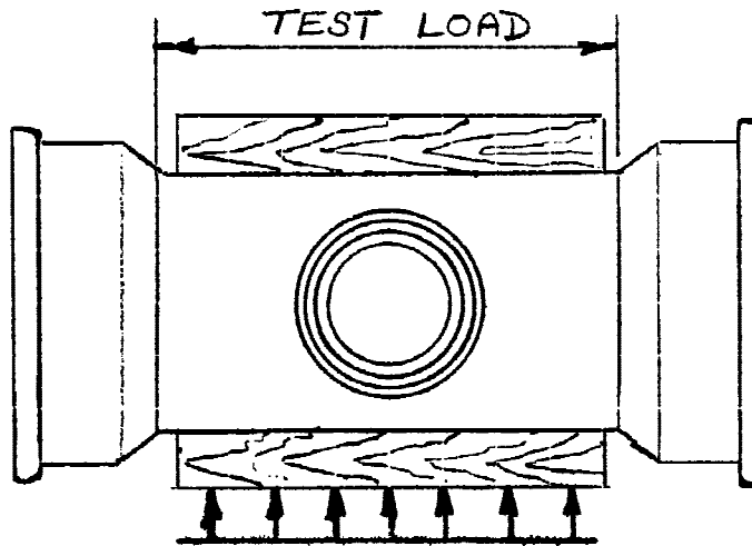
Fitting Body FIG. 1 Length: For blends use center line length. (Blocks shall be 2 in. shorter than body length.)
