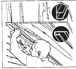
NOTE 1—Apply the vinyl components over the existing unit. FIG. 35 Installation of Soffit on Enclosed Rafter
