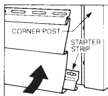
FIG. 12 Fastening of Initial Siding Panel
