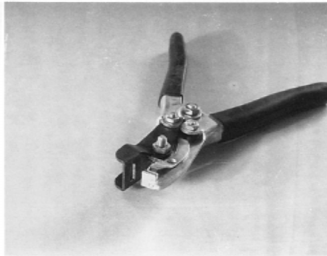
FIG. 3 Nailslot Punch
