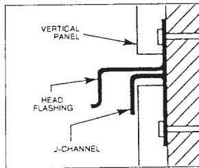
FIG. 28 Joining Area-Multicourse Installation
