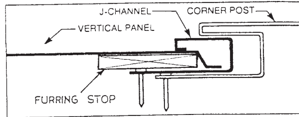
FIG. 31 Installation of Panel Cut-in Bottom of V-Groove
