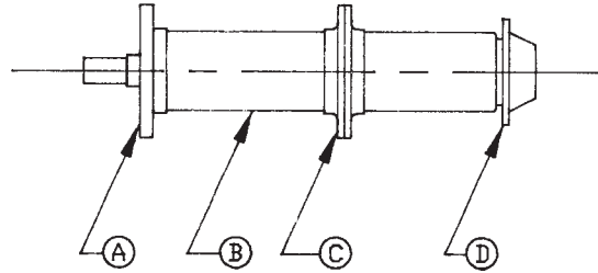
A—End, plate, end cap, or quick closure with coupling for pressure source/vent line. B—Reinforced thermosetting resin pipe (RTRP). C—Test flange set. D—End plate, end cap, or quick closure.
