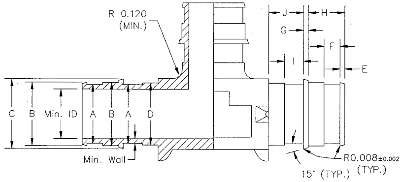
FIG. 2-S Polysulfone Insert Dimensions and Tolerances
