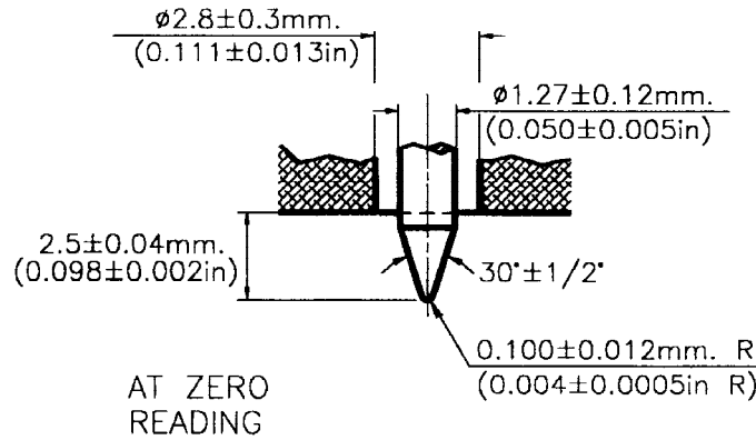
FIG. 1 (b) Type B and D Indentor (continued)
