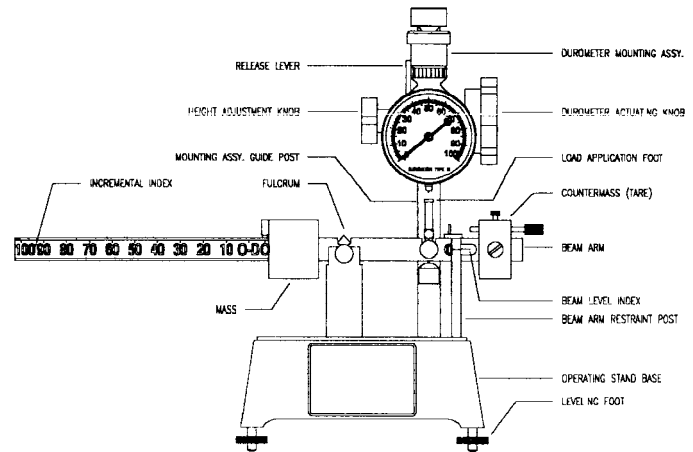
FIG. 5 Example of Durometer Calibration Apparatus
