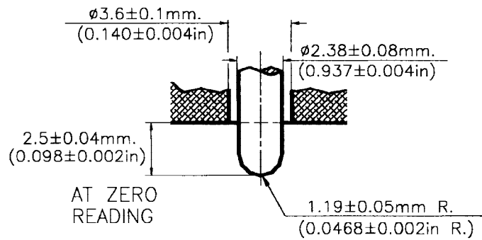
FIG. 1 (c) O, DO, and oo Indentor (continued)
