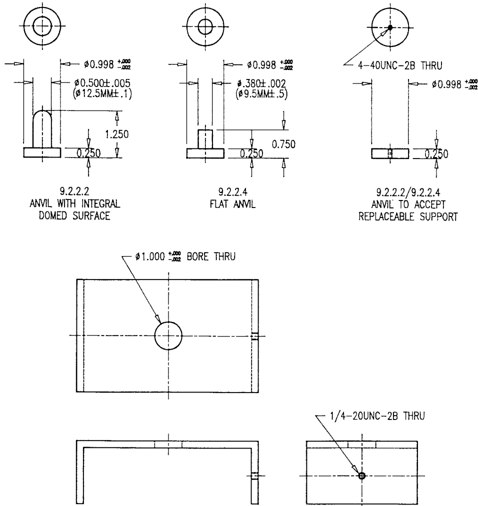
FIG. 3 Bradnick-Warner Support Fixture with Replaceable Anvils
