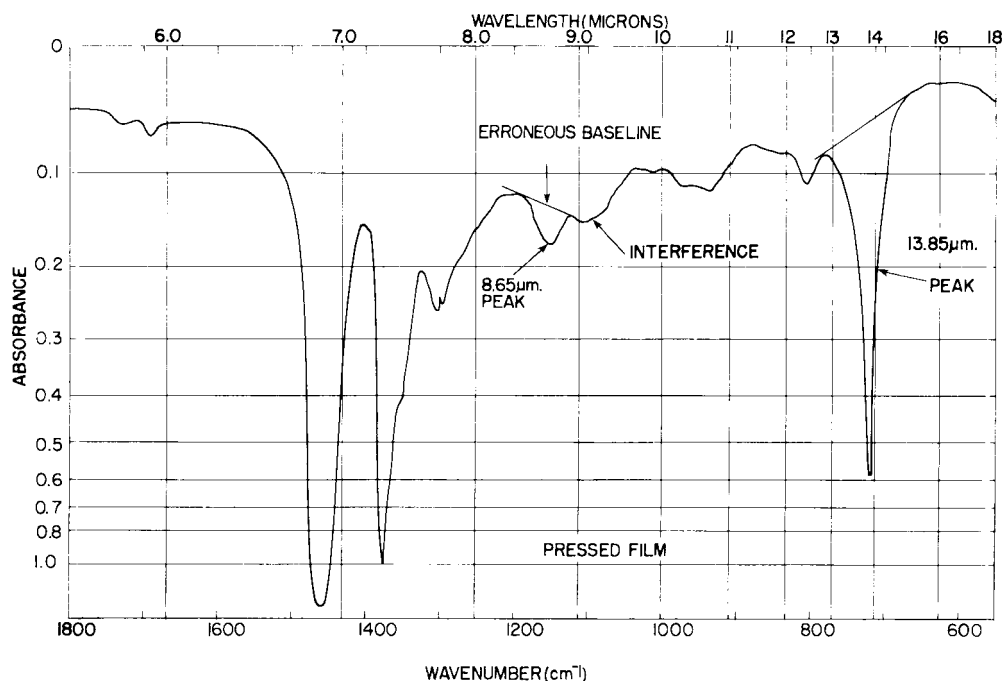
FIG. 1 Illustration of Interference With 8.65- \mu\text{m} Peak
