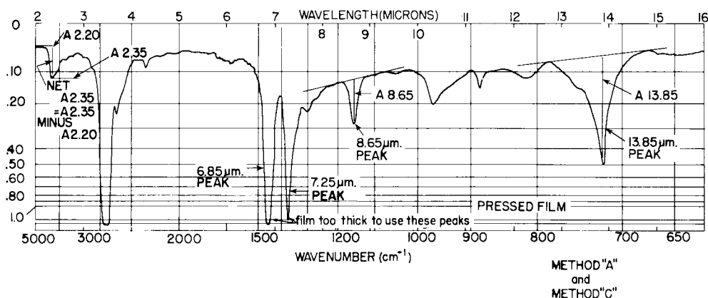
FIG. 2 Baselines for 2.35, 8.65, and 13.85 μm
