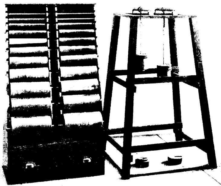
FIG. 2 Mandrels and Frame for Static Mass Adhesion Test
