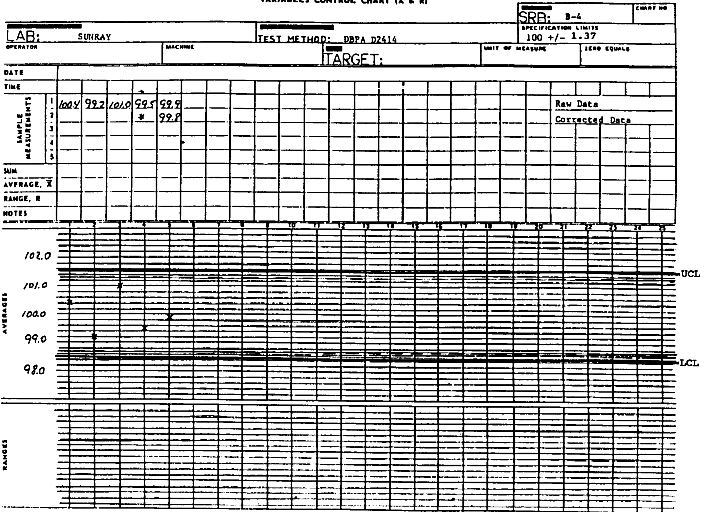
FIG. 2 Control Chart SRB B-4
