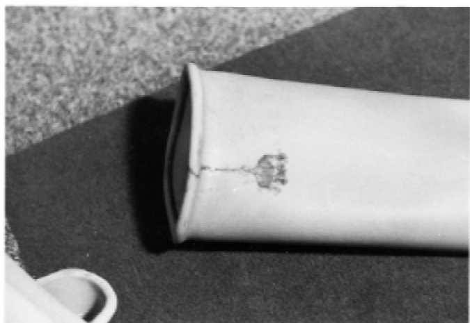
FIG. 26 Tracking—Contaminated Dielectric Fluid
