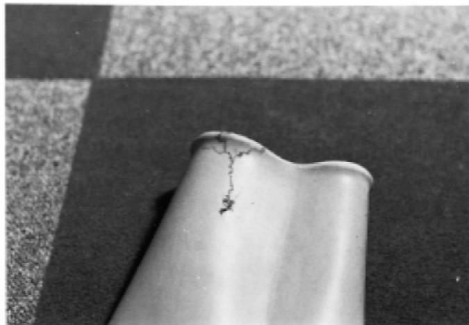
FIG. 25 Tracking—Insufficient Immersion Depth
