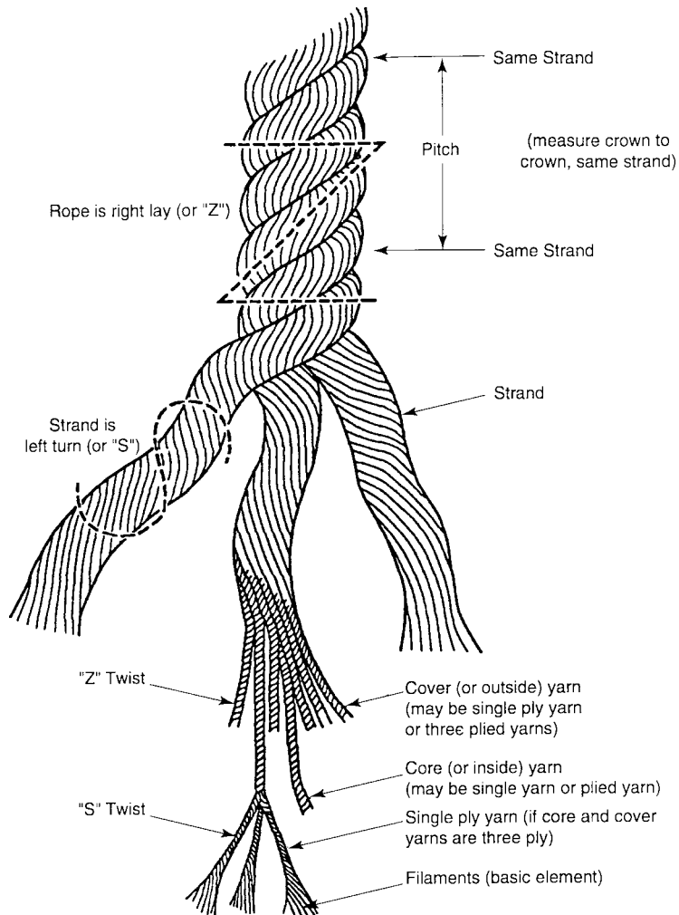
FIG. 1 Polypropylene Rope With Special Electrical Properties
