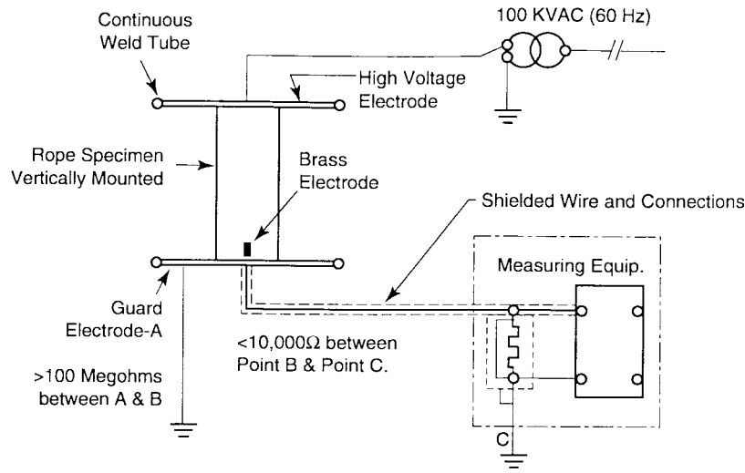
Typical A-C Test Set Up
