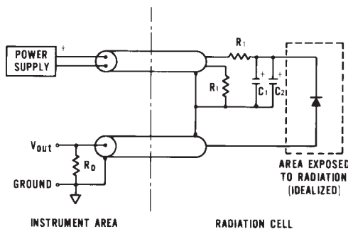
FIG. 2 Irradiation Pulse-Shape Monitor Circuit for Diodes
