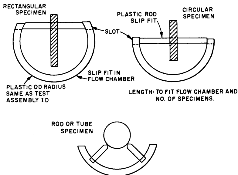
FIG. 3 Specimen Mounts for Flow Chamber
