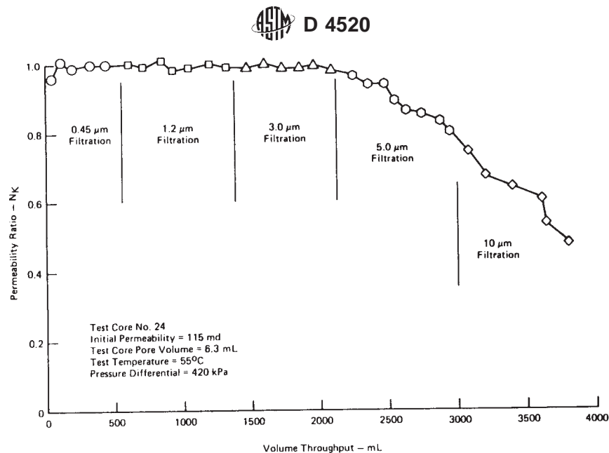
FIG. 4 Example of Filtration Test Results
