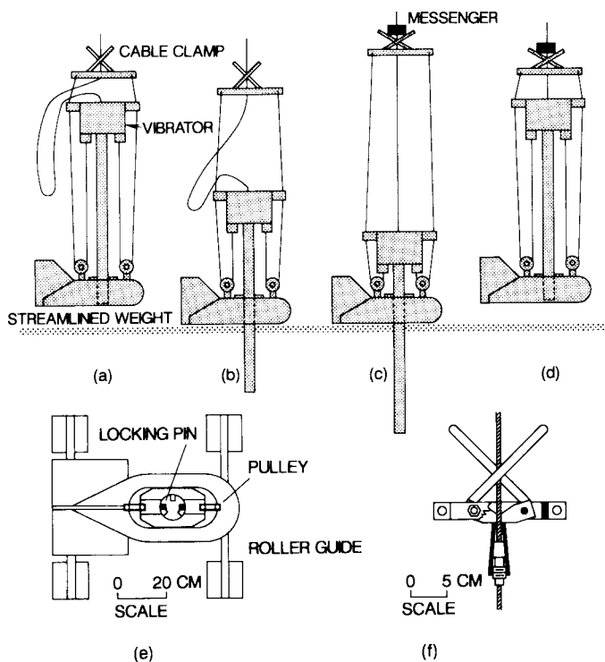
NOTE 1—(a) lowering, (b) coring, (c) extracting, (d) ascending, (e) top view of streamlined weight, and (f) detail of cable clamp.
