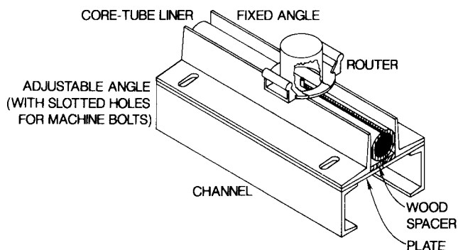
NOTE 1—Fixed angle, plate, and two channels are welded as a unit. FIG. 23 Core-Liner Slitting Apparatus (34)
