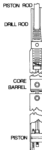
FIG. 14 Butter's Thin-Wall Fixed-Piston Sampler (23)
