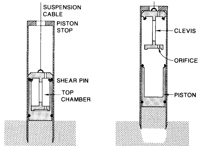
FIG. 5 Release Mechanism
