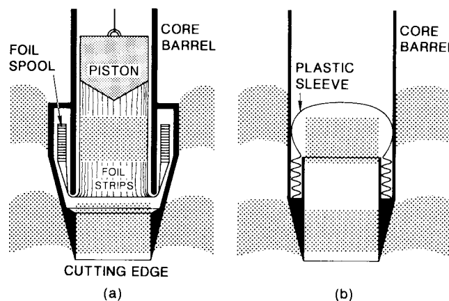
FIG. 3 Core Catchers
