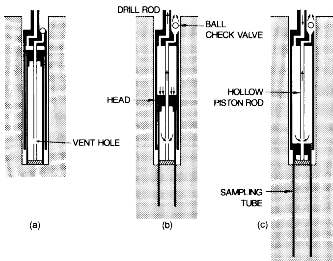
NOTE 1—(a) Retracted sampling tube, (b) partially extended sampling tube, and (c) fully extended sampling tube. (Arrows indicate water flow.)
