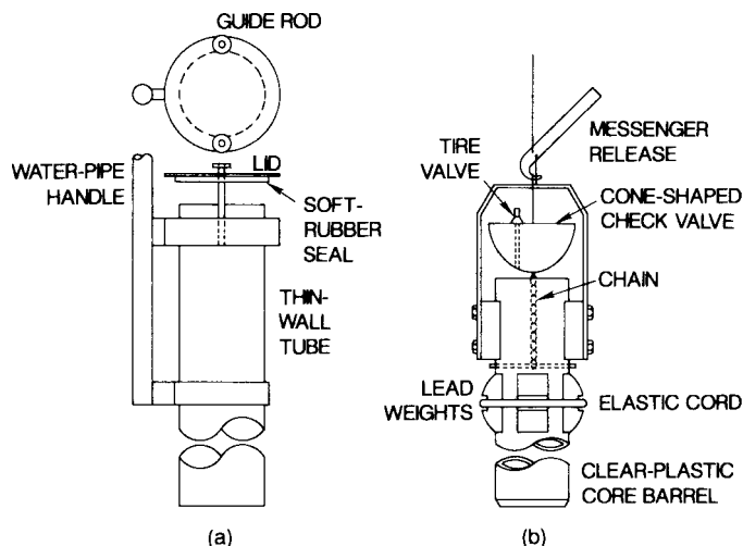
NOTE 1—(a) Modified Van-Stratten sampler. (4) (b) Milbrink's bottom sampler. (6)
