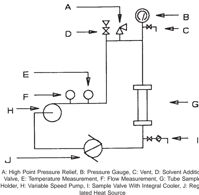
FIG. 3 Dynamic Test Equipment
