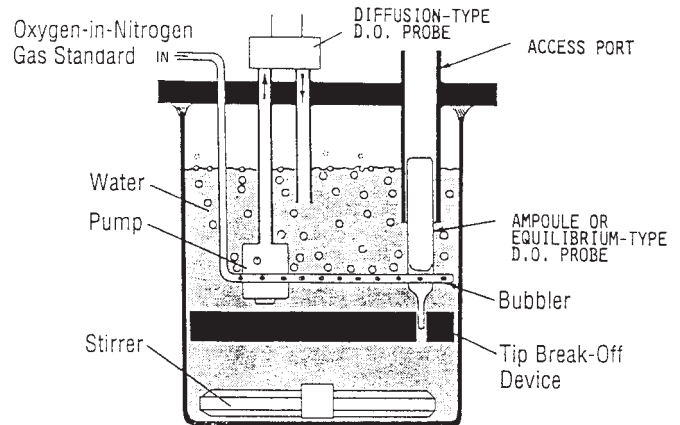
FIG. X2.1 Apparatus for Off-Line Calibration
