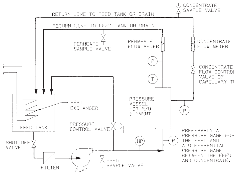
P - PRESSURE TAP LOCATION T - TEMPERATURE MEASUREMENT LOCATION HP - HIGH PRESSURE SHUTOFF PROBE LOCATION
