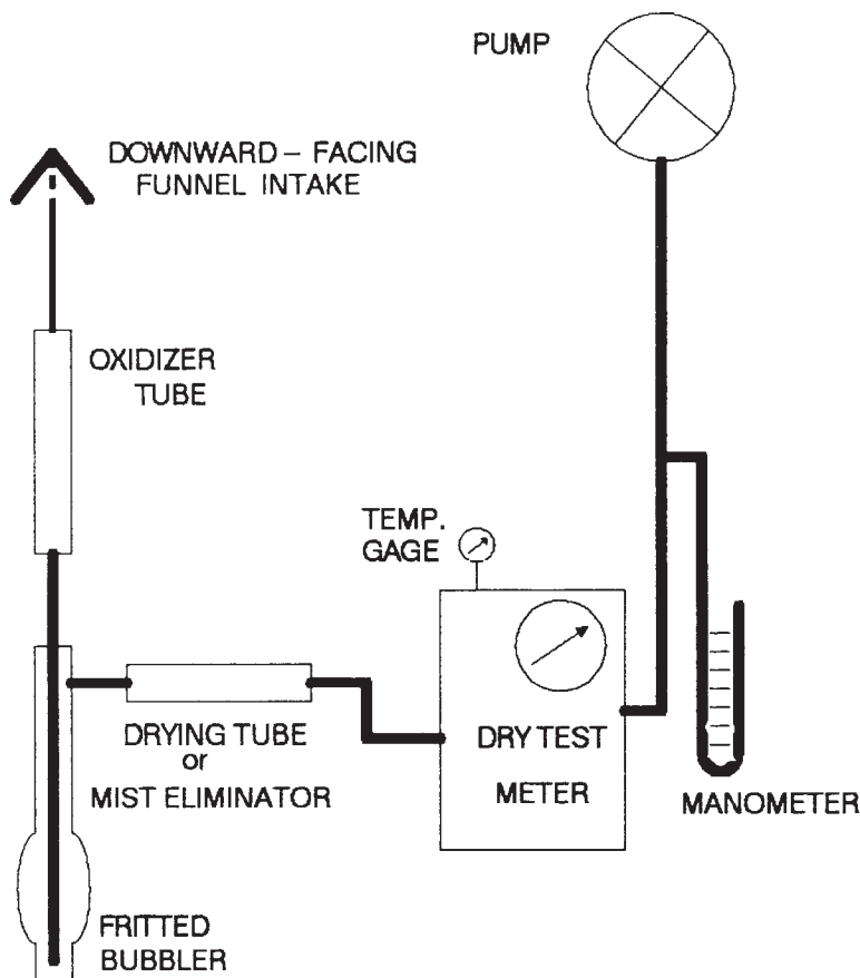
FIG. 2 Sampling Train
