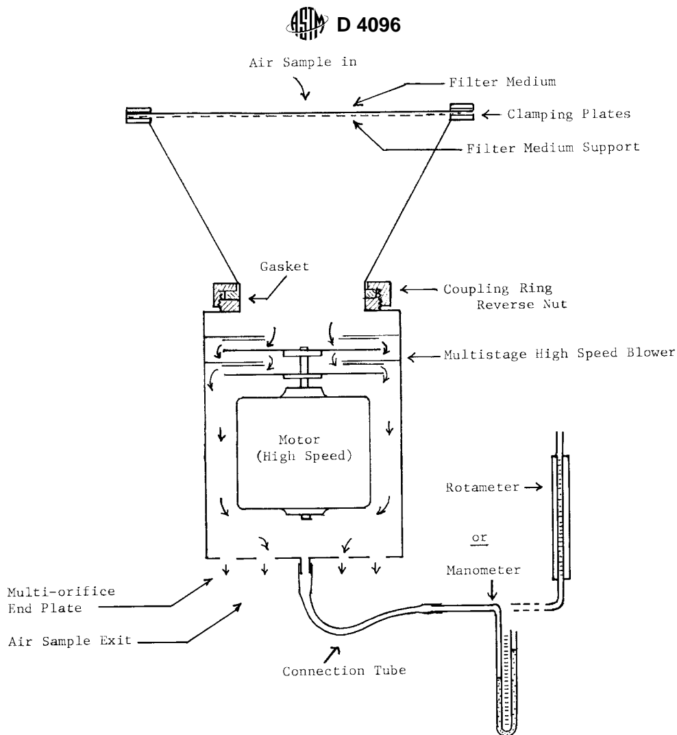
FIG. 2 Schematic Section of a Typical High-Volume Sampler
