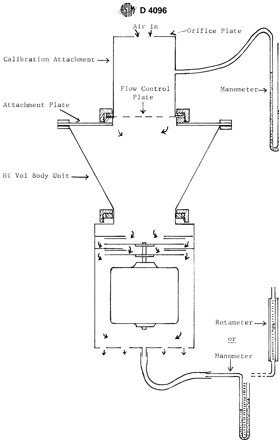
FIG. A1.2 Schematic Section Showing Use of Calibration Attachment Filter Holder Mount
