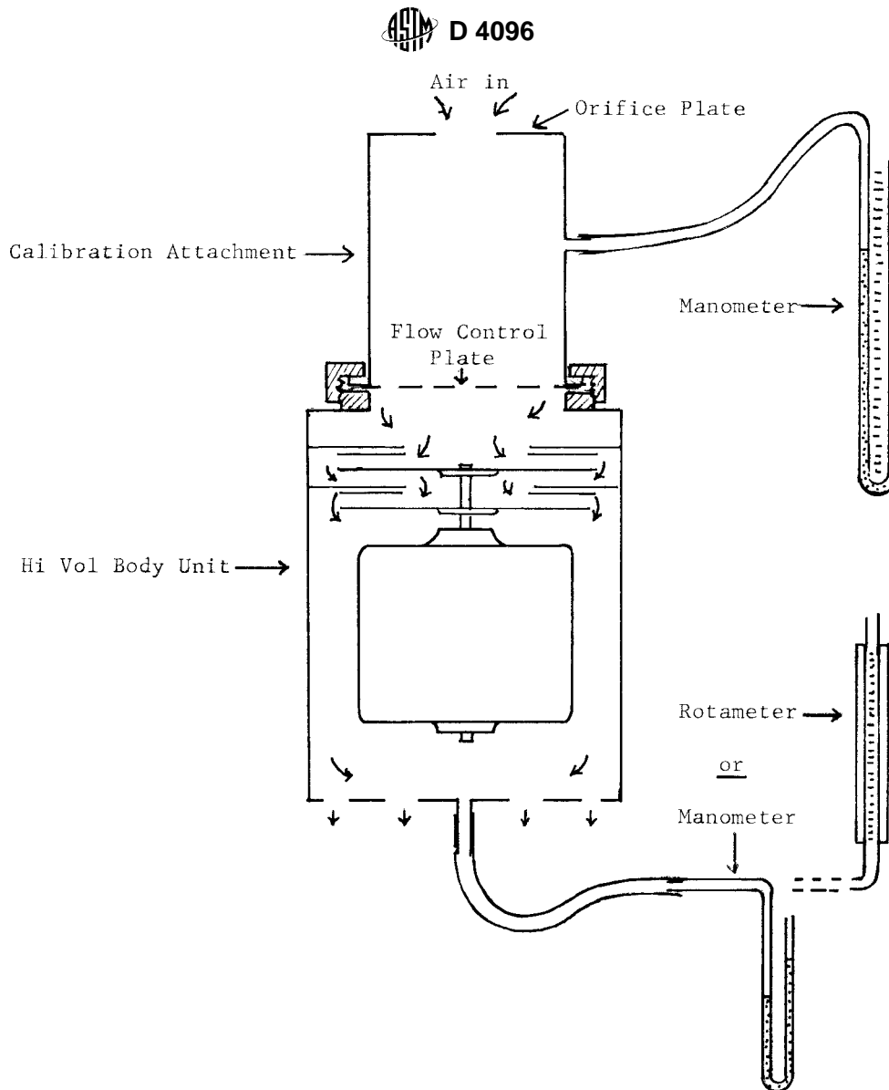
FIG. A1.1 Schematic Section Showing Use of the Calibration Attachment Blower Housing Mount
