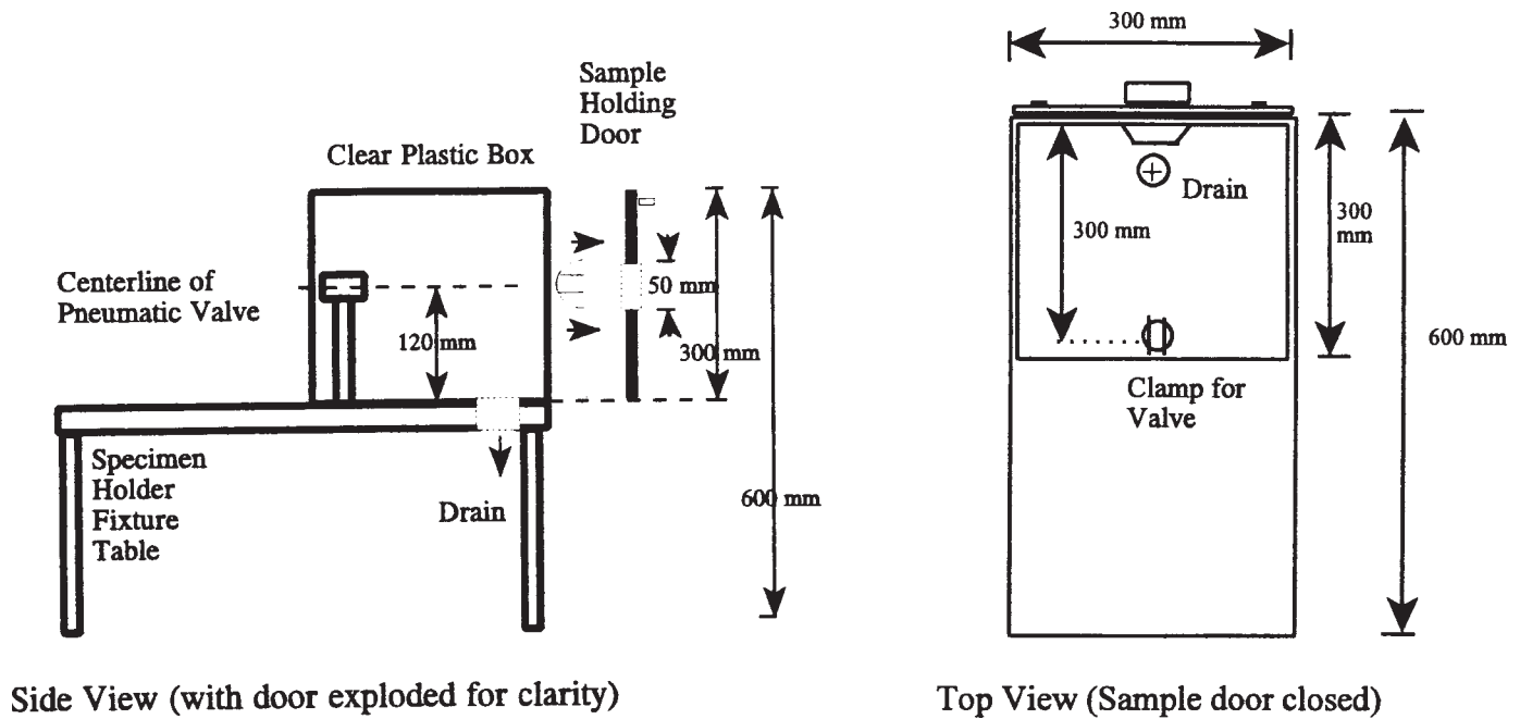
FIG. 2 Specimen Holding Fixture
