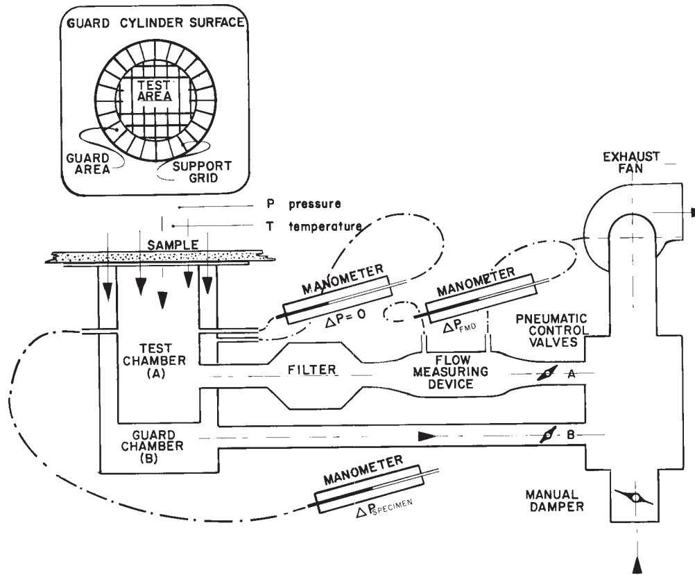
FIG. 3 Method B—Guarded Cylinder Principle
