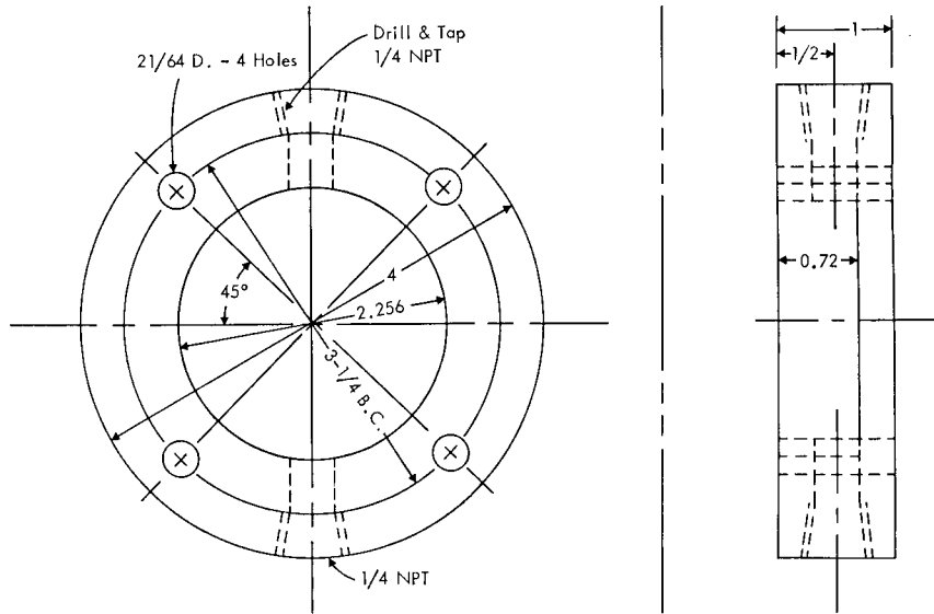
FIG. 4 Cell Body. Penetration Tester ASTM Committee F23.3, Material PTFE, or other suitable for Chemicals Used
