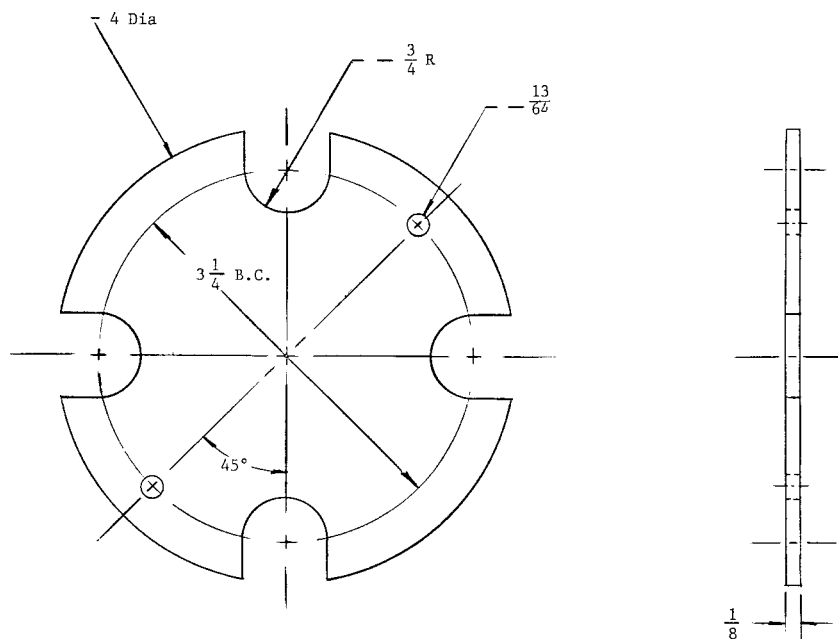
FIG. 9 Optional Transparent Cover for Test Cell Viewing Port
